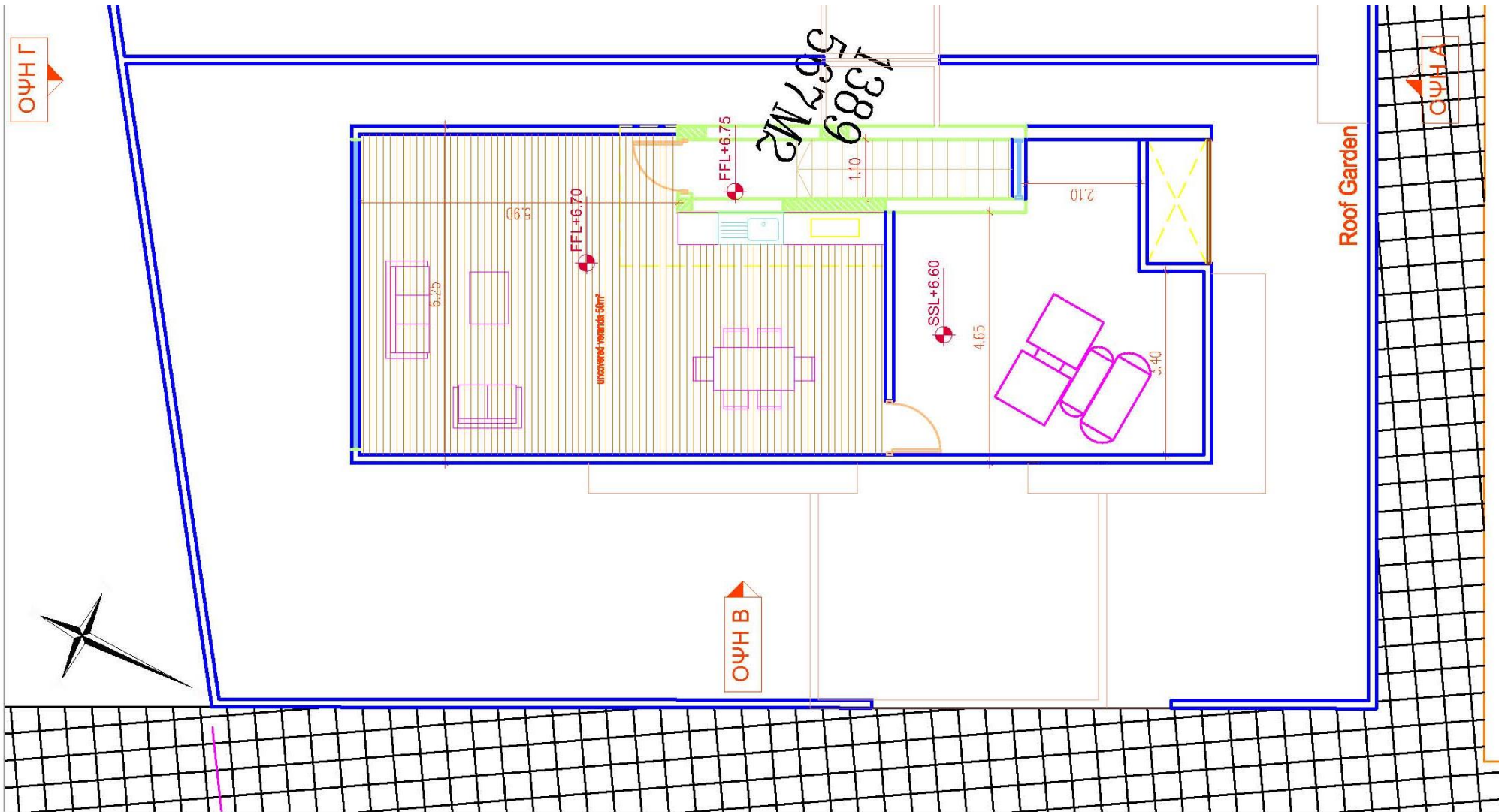
ROOF PLAN OF HOUSE 1
